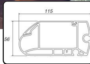
Front Rail
